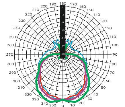
VERTICAL POLAR DIAGRAM — 1400 — 2000 — 2500 — 3150
